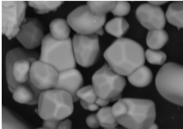
TM-1000_0072 2011/11/21 11:37 D7.7 x6.0k 10 μm
