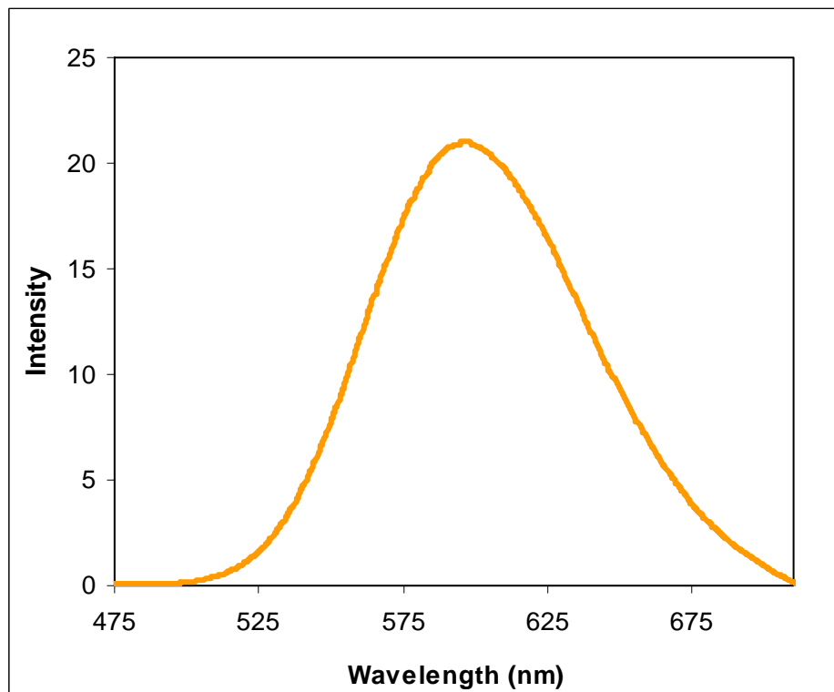
Emission Spectrum
